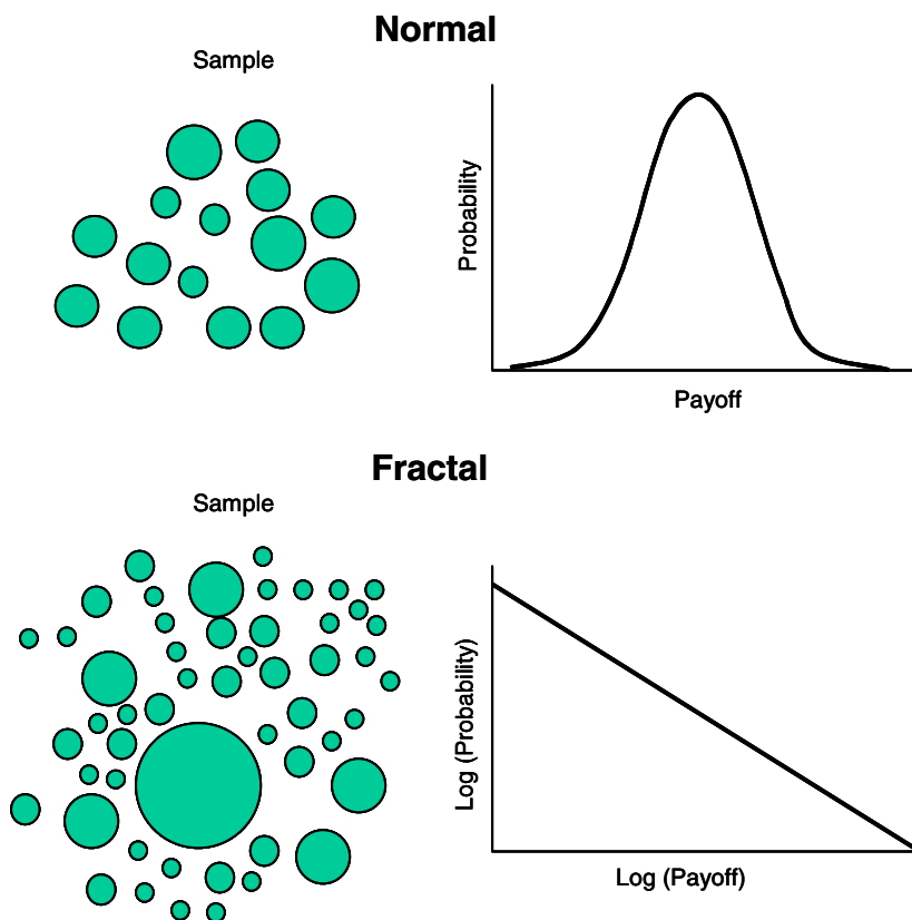
Exhibit 1: Probability Density Functions for Normal and Fractal Systems
